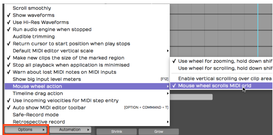
Mouse Wheel MIDI Scrolling Setting
