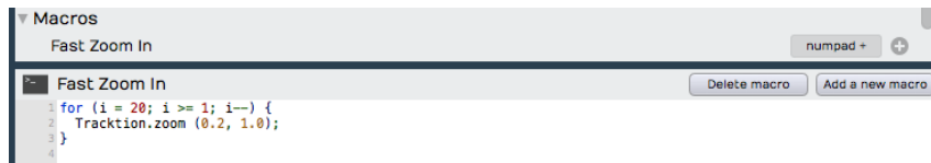
Javascript Macro Example
